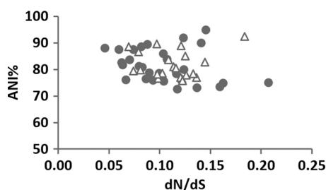
FIG 2 Association between the dN/dS ratio and genomic distance as measured by percent ANI. Closed circles represent bacterial pairs ( n = 28 ), and open triangles represent archaeal pairs ( n = 21 ).
