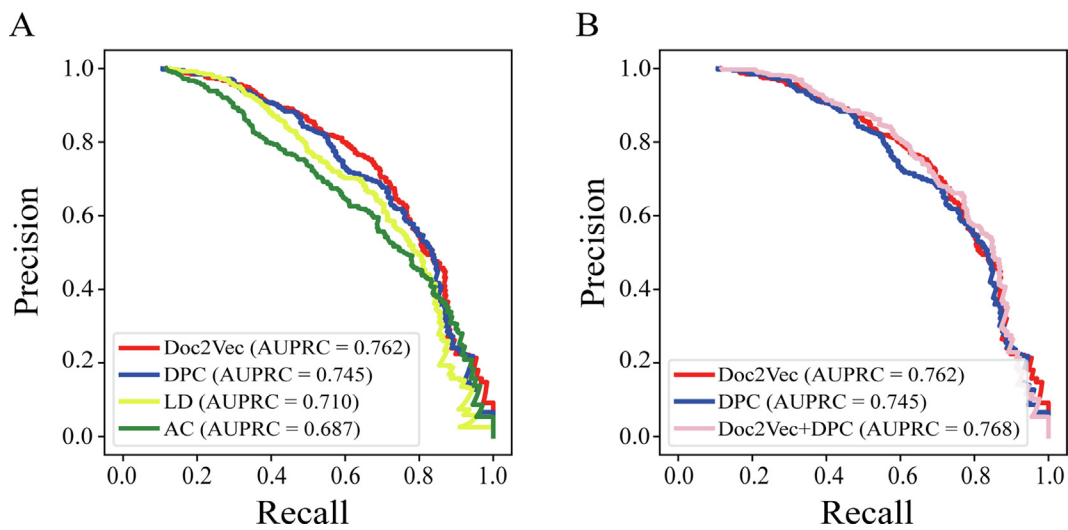
Fig. 2. (A) Performance of different individual sequence encoding schemes-based Random Forest (RF) classifiers in predicting P. falciparum PPIs. Areas under the Precision-Recall curves (AUPRC) indicate that Document to Vector (Doc2Vec) outperformed Di-peptide composition (DPC), Local Descriptor (LD), and Auto Covariance (AC) applying an independent test set. (B) Performance of two best individual sequence encoding schemes (i.e., Doc2Vec and DPC)-based RF classifiers and their sequence encoding combination (Doc2Vec + DPC)-based RF classifier in predicting P. falciparum PPIs. AUPRC indicates that the combination sequence encoding scheme slightly outperformed each individual sequence encoding scheme.
