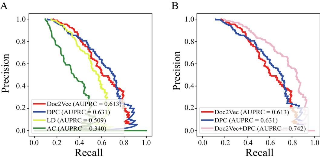
Fig. 3. (A) Performance of different individual sequence encoding schemes-based Random Forest (RF) classifiers in predicting P. falciparum PPIs based on the novel partition of the dataset (i.e., non-overlapped proteins between the training set and test set). Areas under the Precision-Recall curves (AUPRC) indicate that Di-peptide composition (DPC) outperformed Document to Vector (Doc2Vec), Local Descriptor (LD), and Auto Covariance (AC) applying an independent test set. (B) Performance of two best individual sequence encoding schemes (i.e., DPC and Doc2Vec)-based RF classifiers and their combination (Doc2Vec + DPC)-based RF classifier in predicting P. falciparum PPIs. AUPRC indicates that the sequence encoding scheme combination significantly improves the performance compared to each sequence encoding scheme.
