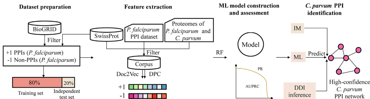
Fig. 1. Workflow of the proposed computational pipeline to predict C. parvum PPIs. In the dataset preparation step, we constructed positive and negative samples based on P. falciparum PPI data from BioGRID as well as the Swiss-Prot database and divided the dataset into a training set (80%) and an independent test set (20%). Furthermore, we extracted protein features using the Doc2Vec encoding scheme and DPC encoding scheme. The Doc2Vec model was trained on the compiled protein corpus covering sequences from Swiss-Prot, P. falciparum PPI dataset, and proteomes of P. falciparum and C. parvum . Based on the encoded feature vectors of the P. falciparum PPI dataset, we further trained the ML classification model using the RF algorithm and assessed the model's performance. Finally, we transferred the trained ML model to predict C. parvum PPIs and combined two other traditional methods (i.e., IM and DDI inference) to obtain the high-confidence C. parvum PPI network.
